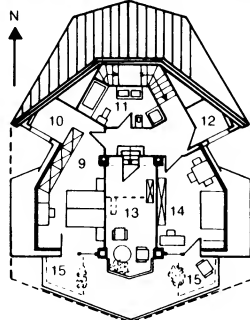
10 Plan view - upper floor
